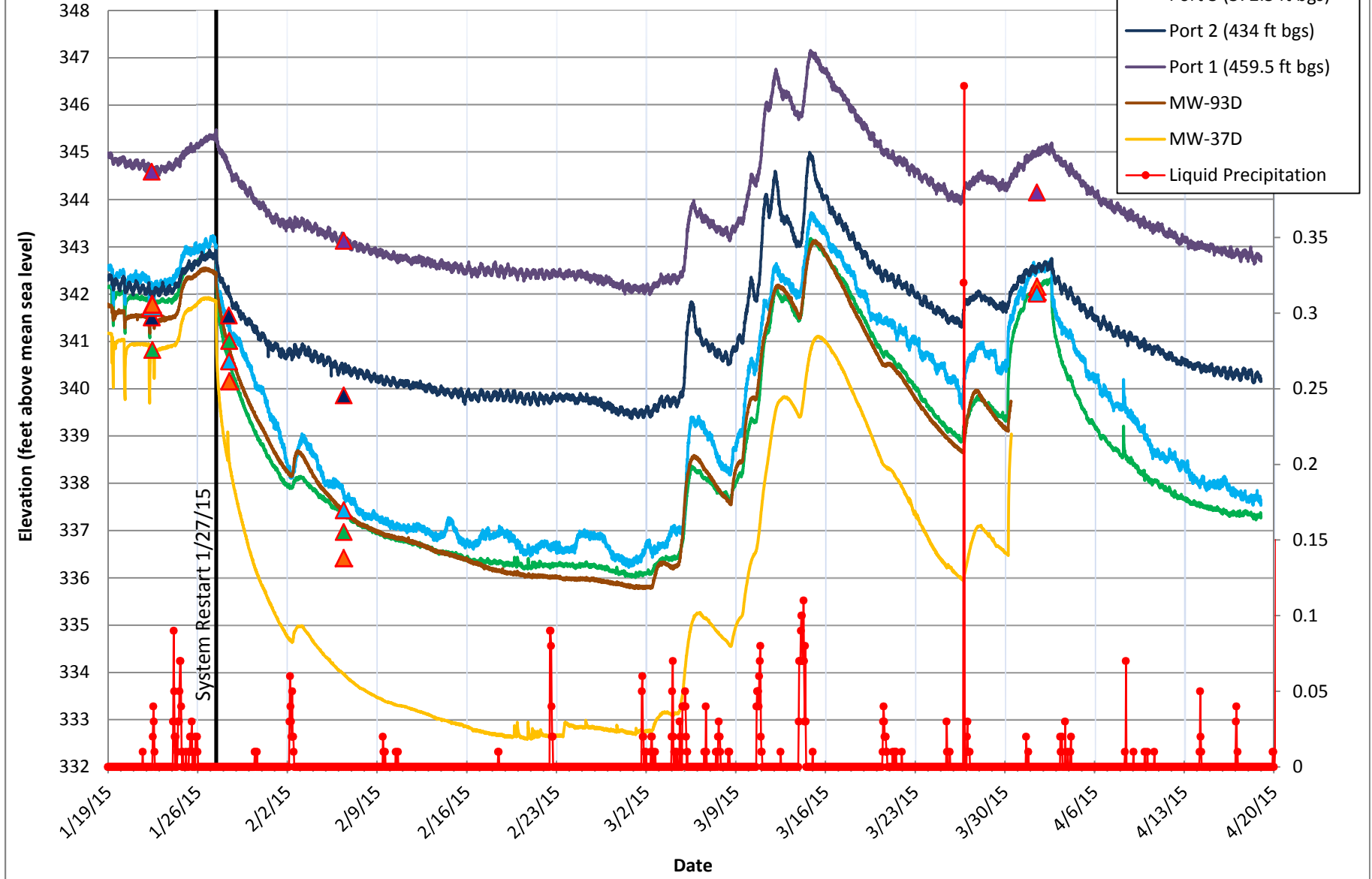
Figure 3.5-16 MW-136A Potentiometric Elevations
